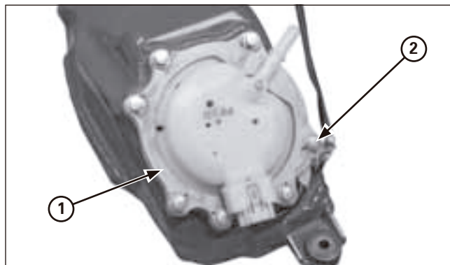
(1) SUPPORT DE LA POMPE ESSENCE (2) VIS
